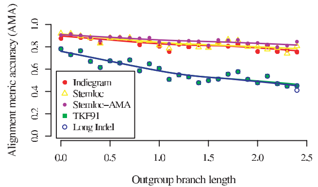
Figure 11. Dependence of alignment metric accuracy on alignment method and outgroup branch length. We simulated the evolution of three structural RNAs under the TKFST model. The simulation included two sister species at unit distance from the ancestral sequence, plus one “outgroup” whose branch length t was varied between [0, 2.5] by selecting 25 equally spaced values of t in this range, spaced 0.1 apart. We then simulated 25 alignments for each value of t , using TKFST model parameters described in the text. The Alignment Metric Accuracy (AMA) is, roughly, the proportion of residues that are correctly aligned, averaged over all pairs of sequences (see [54] for a precise definition; we set the AMA Gap Factor to 1). The AMA between the true alignment and the inferred alignment was measured for various statistical alignment inference procedures. These procedures are described in the text, but may be summarized very briefly as ML under the true model (“Indiegram”); greedy approximate-ML progressive alignment by single-linkage clustering with pair SCFGs (“Stemloc”); sequence annealing, a form of posterior decoding to maximize a sum-over-pairs accuracy metric, using pair SCFGs to get the posterior probabilities (“Stemloc-AMA”); statistical alignment using the TKF91 model, i.e. linear gap-penalties (“TKF91”); and statistical alignment using a long-indel model, i.e. affine gap-penalties (“Long Indel”). doi:10.1371/journal.pcbi.1000483.g011
