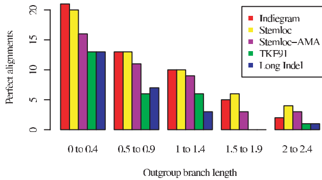
Figure 10. Dependence of perfect alignment rate on alignment method and outgroup branch length. Perfect alignment is when a given alignment program estimates the alignment 100% correctly, with no errors. Simulating the evolution of three structural RNAs under the TKFST model, we investigated the dependency of perfect alignment rate on outgroup branch length. The simulation included two sister species at unit distance from the ancestral sequence, plus one “outgroup” whose branch length t was varied between [0, 2.5] by selecting 25 equally spaced values of t in this range, spaced 0.1 apart. (A unit-length branch here corresponds to one expected substitution per site in loop sequence.) We simulated 25 alignments for each value of t , using TKFST model parameters described in the text. Since the perfect alignment rate is rather low, we further aggregated the t -values into bins of five; thus, for example, the bin named “0 to 0.4” includes t \in \{0.0, 0.1, 0.2, 0.3, 0.4\} and represents 25 \times 5 = 125 trials in total. The perfect alignment rate was measured for various statistical alignment inference procedures. These procedures are described in the text, but may be summarized very briefly as ML under the true model (“Indiegram”); greedy approximate-ML progressive alignment by single-linkage clustering with pair SCFGs (“Stemloc”); sequence annealing, a form of posterior decoding to maximize a sum-over-pairs accuracy metric, using pair SCFGs to get the posterior probabilities (“Stemloc-AMA”); statistical alignment using the TKF91 model, i.e. linear gap-penalties (“TKF91”); and statistical alignment using a long-indel model, i.e. affine gap-penalties (“Long Indel”). doi:10.1371/journal.pcbi.1000483.g010
