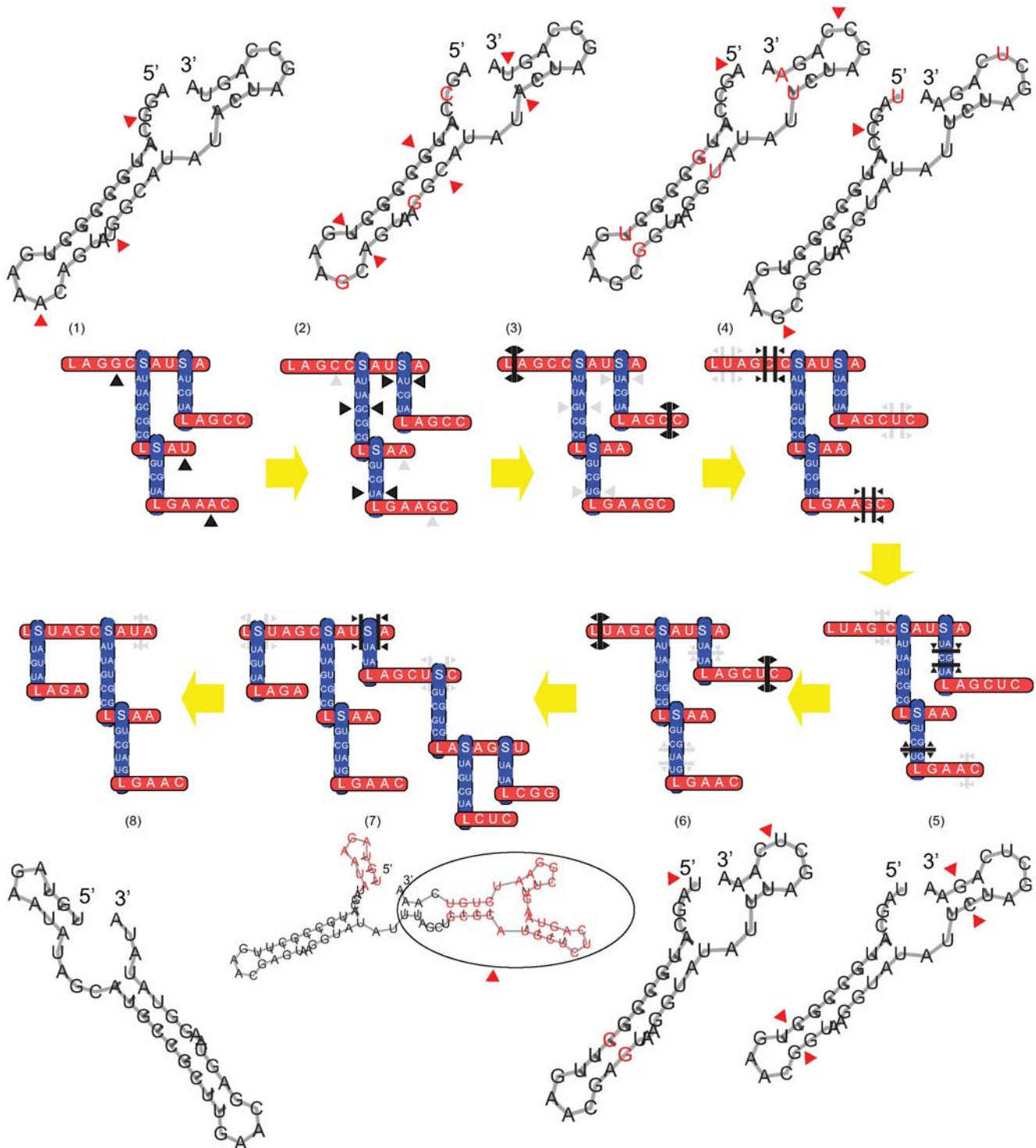
Figure 9. Evolution of a RNA structure under the TKF Structure Tree model. The TKF Structure Tree model includes phenomena such as point mutations in loop sequences (1→2 and 4→5), covariant mutations in stem sequences (2→3), insertions in loop sequences (3→4), insertions in stem sequences (5→6), structural insertions (6→7), and structural deletions (7→8). Figure is extended from a similar version in [29]. doi:10.1371/journal.pcbi.1000483.g009
