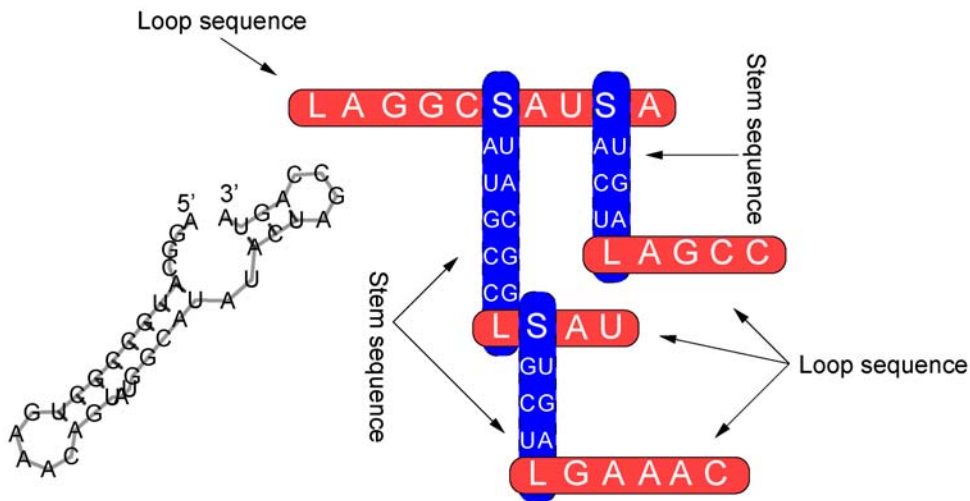
Figure 8. The TKF Structure Tree model represents the evolution of RNA structure as nested stem and loop sequences. The model consists of recursively nested loop sequences (gray, horizontal) and stem sequences (black, vertical). The loops are sequences of unpaired bases and the stems are sequences of covarying base-pairs. Both loop and stem sequences evolve according to the Thorne-Kishino-Felsenstein (TKF) model [44] of molecular evolution. Figure is extended from a similar version in [29]. doi:10.1371/journal.pcbi.1000483.g008
