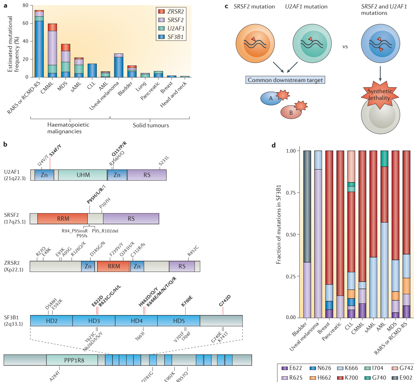
Figure 2 | Commonly mutated spliceosomal proteins and their associations with specific cancer types. a | The incidence and cancer distribution of the most frequently mutated spliceosomal genes are shown. b | The spectrum of mutations that have been identified in U2 small nuclear RNA auxiliary factor 1 (U2AF1), serine/arginine-rich splicing factor 2 (SRSF2), zinc finger, RNA-binding motif and serine/arginine-rich 2 (ZRSR2) and splicing factor 3B, subunit 1 (SF3B1). Mutations shown in bold text occur at hot spots; other illustrated mutations are recurrent but rare. As ZRSR2 mutations do not occur at hot spots, very rare or private mutations are shown as examples. c | Schematic illustrating the potential reasons that spliceosomal gene
