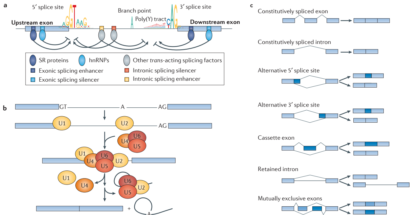
Figure 1 | Simplified model of constitutive and alternative splicing. a | The key sequence features that govern splicing are shown, including consensus sequences of the 5' and 3' splice sites and sequence motifs bound by trans -acting splicing factors (serine/arginine-rich (SR) proteins, heterogeneous nuclear ribonucleoproteins (hnRNPs) and others). Sequence elements required for assembly of the spliceosome onto the pre-mRNA, including the splice sites themselves, polypyrimidine (poly(Y)) tract and branch point, frequently follow the illustrated consensus motifs, whereas the sequences of enhancer or silencer elements depend upon the specific RNA-binding protein that recognizes them. Consensus motifs are illustrated as sequence logos, in which the height of each nucleotide corresponds to its approximate genome-wide frequency in bits. Sequence motifs are illustrated as genomic DNA sequence rather than pre-mRNA sequence (T instead of U). Note that splicing factors such as SR proteins and hnRNPs frequently have context-dependent regulatory roles. b | Simplified schematic of intron excision and ligation of two adjacent exons. The steps shown are: recognition of the 5' and 3' splice sites by the U1 and U2 small nuclear ribonucleoprotein complexes (snRNPs), assembly of the snRNPs into the active spliceosome, excision of the intron lariat and ligation of the two exons. c | Schematic of constitutive and alternative splicing events. Light blue: constitutive sequence that always forms part of the mature mRNA; mid-blue or dark blue: alternative sequence that can be either included or excluded in the mature mRNA.
