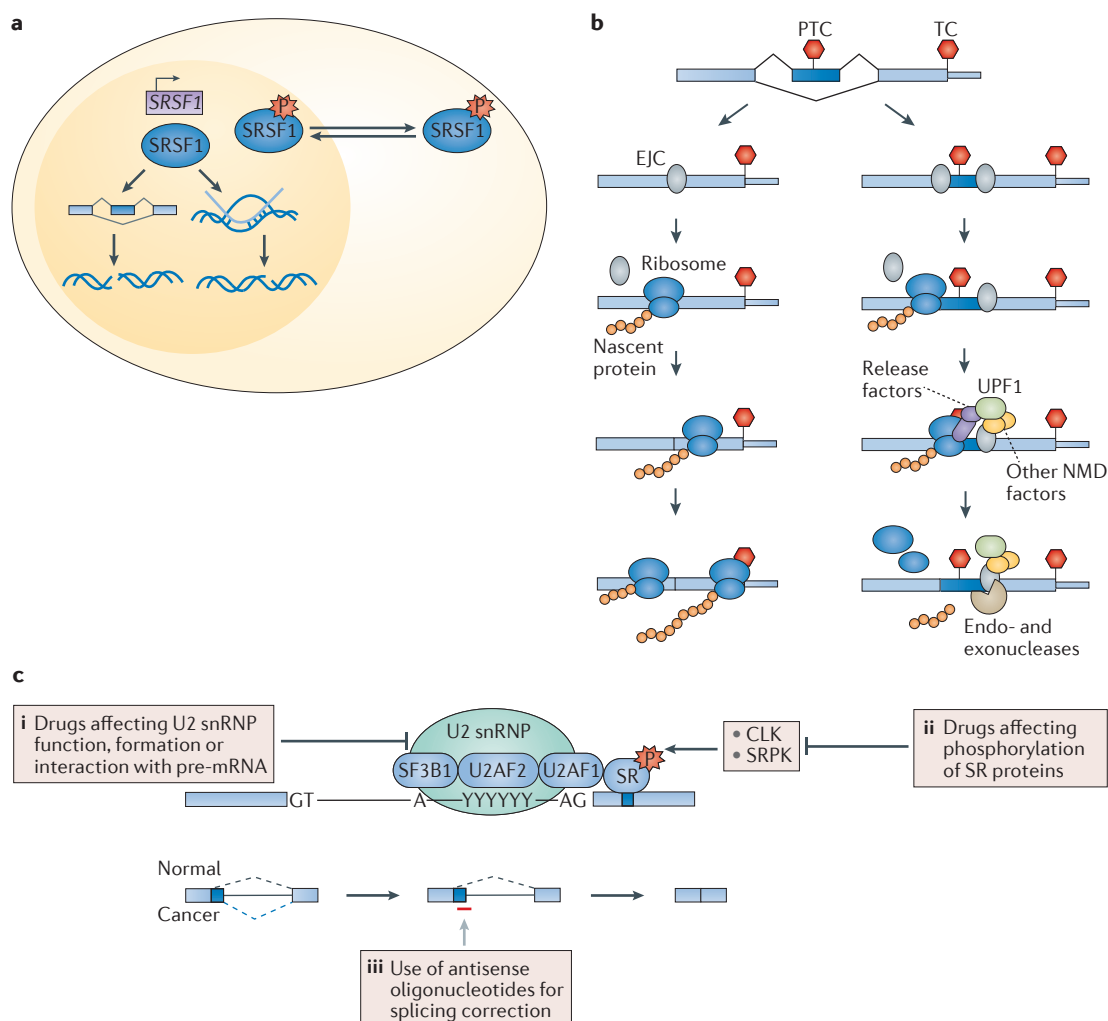
Figure 4 | Links between splicing factors and diverse biological processes and potential methods for therapeutic manipulation of splicing. a | Changes in the abundance, post-translational modifications and/or subcellular localization of splicing factors such as serine/arginine-rich splicing factor 1 (SRSF1) can cause DNA damage or influence the DNA damage response (DDR). Splicing factors have been linked to DNA damage and the DDR both directly (for example, insufficient levels of splicing factors can cause R loop formation and genomic instability) and indirectly (for example, through downstream changes in splicing). b | The steps involved in nonsense-mediated decay (NMD) are shown. The exon junction complex (EJC; grey) is deposited upstream of exon-exon junctions on the processed mRNA, and is displaced by the ribosome (blue) during the pioneer (first) round of translation. Ribosome stalling at a premature termination codon (PTC) >50 nt upstream of an EJC promotes interactions between release factors (purple) and up-frameshift suppressor 1 (UPF1; green), recruitment of other NMD components (yellow) and RNA degradation by endo- and exonucleases (beige). In contrast, if only a normal termination codon (TC) is present, then all EJCs are displaced by the ribosome during the pioneer round of translation and NMD is not triggered. Red stop signs indicate stop codons. c | Compounds and oligonucleotides that can disrupt or modulate normal splicing catalysis or alter splice site recognition through distinct pathways include drugs affecting U2 small nuclear ribonucleoprotein (snRNP) function, formation and/or interaction with pre-mRNA (panel i), drugs affecting post-translational modifications of serine/arginine-rich (SR) proteins and potentially other splicing factors (panel ii) and oligonucleotides to manipulate specific mRNA isoforms that may be important in tumour maintenance (panel iii). CLK, CDC2-like kinase; SF3B1, splicing factor 3B, subunit 1; SRPK, SR protein kinase; U2AF, U2 auxiliary factor.
