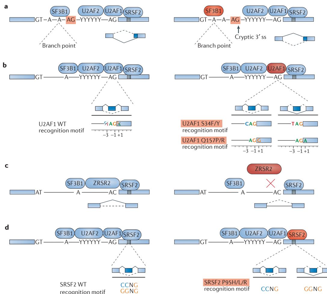
Figure 3 | Current understanding of the mechanistic consequences of spliceosomal gene mutations for RNA splicing. a | Splicing factor 3B, subunit 1 ( SF3B1 ) mutations (mutant form shown in red) alter 3' splice site (ss) selection by permitting or enhancing recognition of cryptic upstream 3' splice sites. It is not yet known how mutations affecting SF3B1 alter its target protein–RNA and/or protein–protein interactions to drive this cryptic splice site recognition. Sequence motifs are illustrated as genomic DNA sequence rather than pre-mRNA sequence (T instead of U). b | U2 small nuclear RNA auxiliary factor 1 ( U2AF1 ) mutations alter 3' ss consensus sequences. Wild-type U2AF1 recognizes the consensus motif yAG|r at the intron–exon boundary (y = pyrimidine, r = purine, | = intron–exon boundary). S34F or S34Y mutations (shown in red) promote recognition of cAG|r over tAG|r, whereas Q157P or Q157R mutations (shown in red) promote recognition of yAG|g over yAG|a. c | Zinc finger, RNA-binding motif and serine/arginine-rich 2 ( ZRSR2 ) mutations (shown in red) cause loss of ZRSR2 function to induce splicing defects, primarily involving the aberrant retention of U12-type introns. d | Serine/arginine-rich splicing factor 2 ( SRSF2 ) mutations (shown in red) alter exonic splicing enhancer preferences. Wild-type SRSF2 recognizes the consensus motif SSNG (S = C or G), whereas mutant SRSF2 preferentially recognizes the CCNG motif over the GGNG motif.
