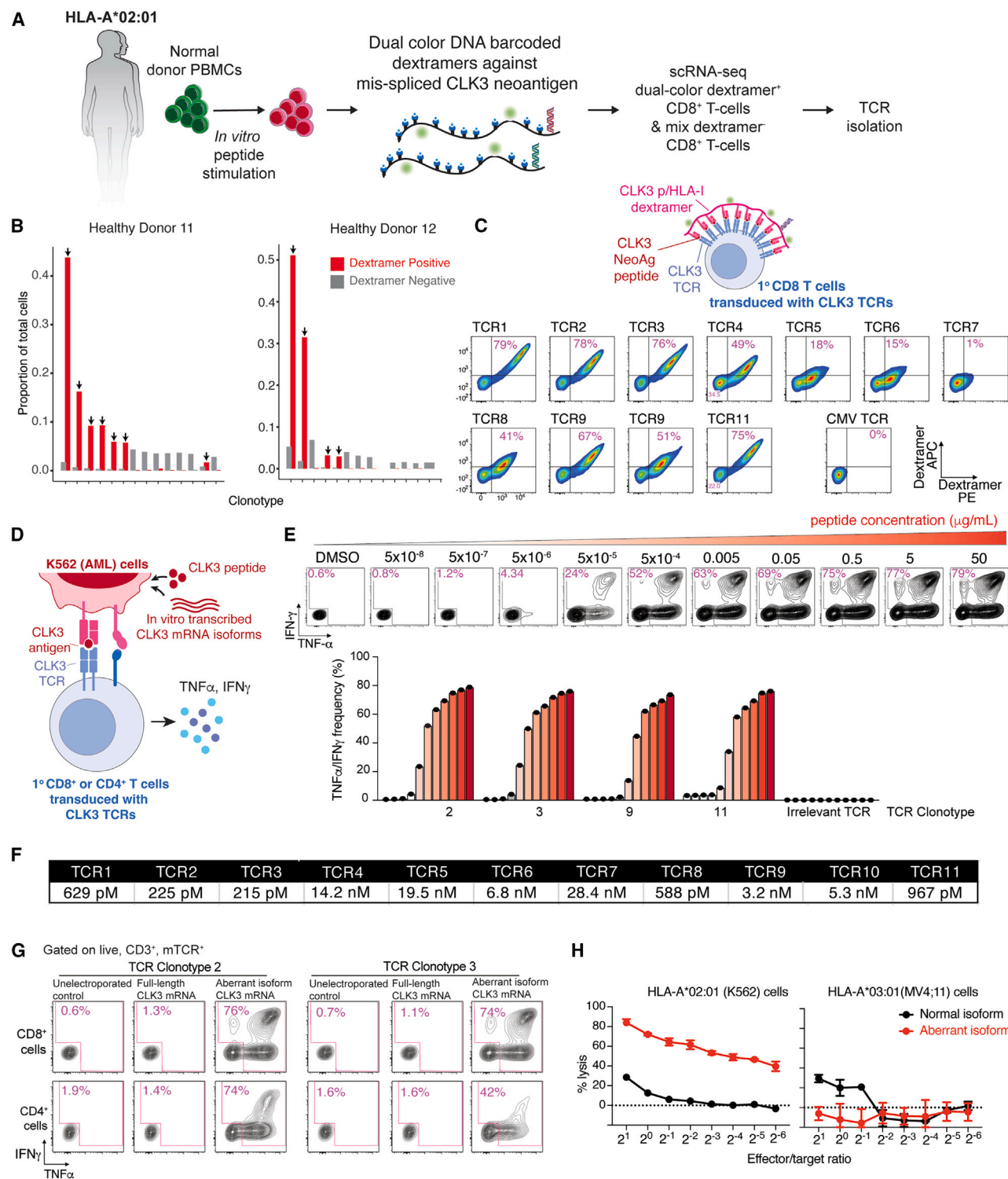
Figure 4. Discovery and characterization of TCRs recognizing the CLK3 neoantigen
