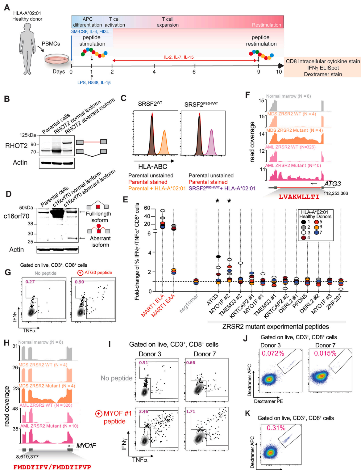
Figure S2. Immunogenicity of candidate SRSF2 or ZRSR2 mutant-induced neoantigens and dextramer-based identification of neoantigen-reactive CD8 + T cells, related to Figure 2
