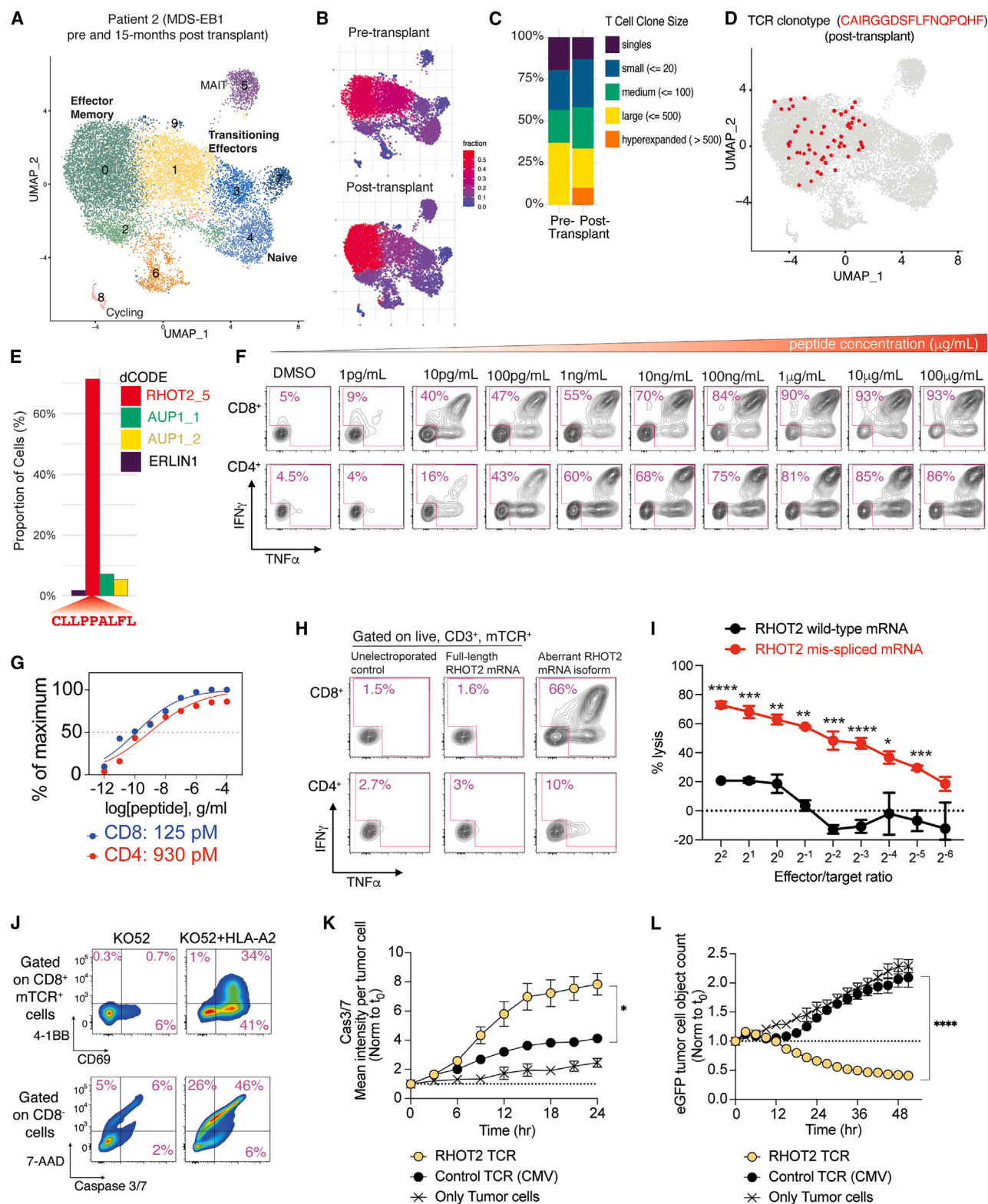
Figure 7. Neoantigen-reactive T cells and TCRs pre and post HLA-matched allogeneic transplantation in splicing factor mutant leukemia patients
