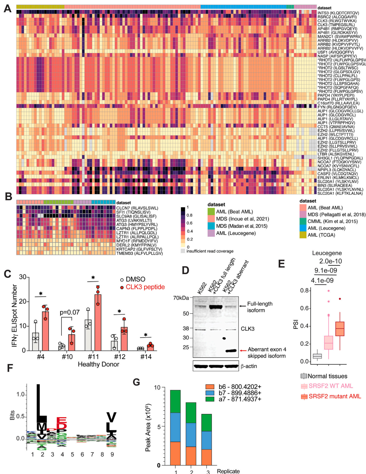
Figure S3. Functional characterization of the CLK3 neoantigen, related to Figure 3
